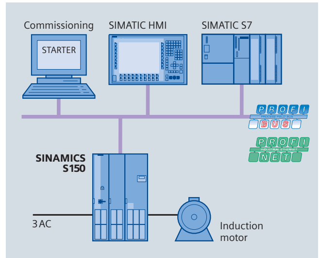
Configuration example: SINAMICS S150 with SIMATIC S7
