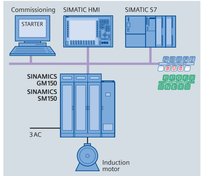
Configuration example: SINAMICS GM150 and SINAMICS SM150 with SIMATIC S7
